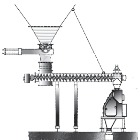
Archimedean screw
