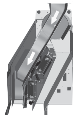
BY-PASS position for flowrate measurement
